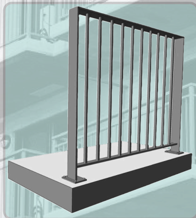
BARROTIN CENTRÉ SOUDÉ BARROTIN CENTRED WELDED
